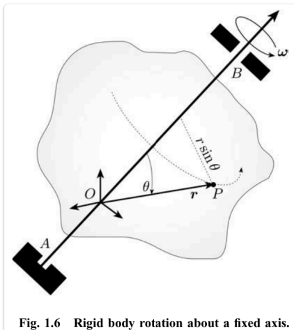
Fig. 1.6 Rigid body rotation about a fixed axis.
