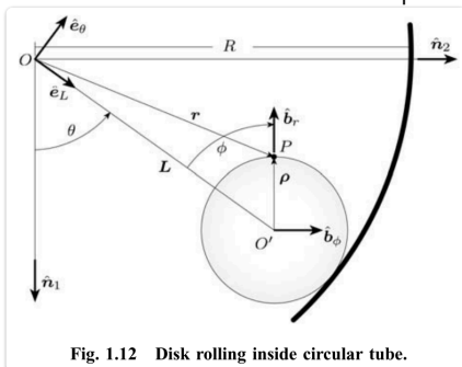
Fig. 1.12 Disk rolling inside circular tube.
