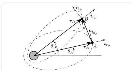
Fig. 1.8 Relative motion of two satellites on coplanar elliptic orbits.
